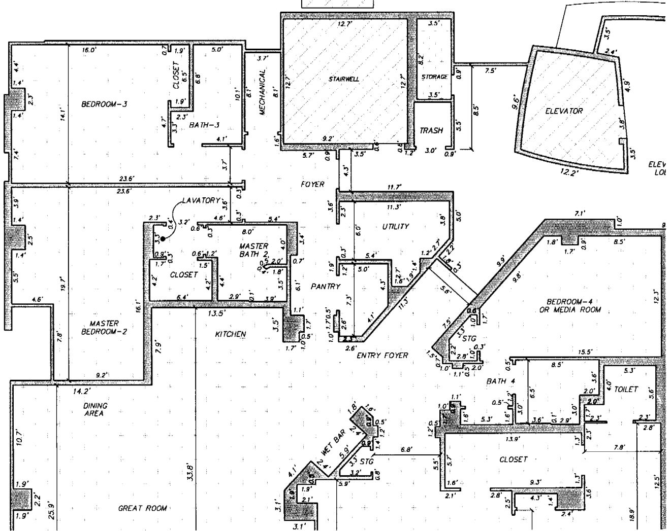
GRAPHIC SCALE 1" = 10'
