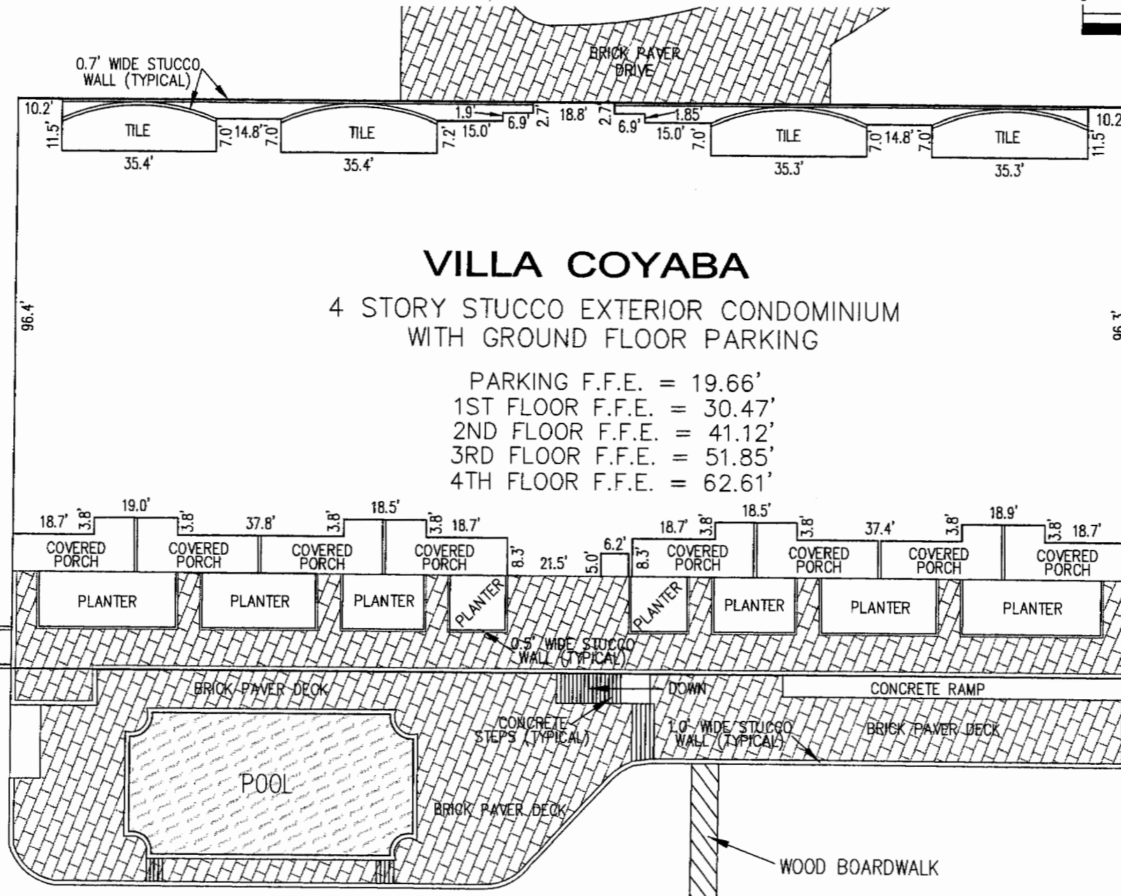
SITE PLAN - DETAIL SHEET
